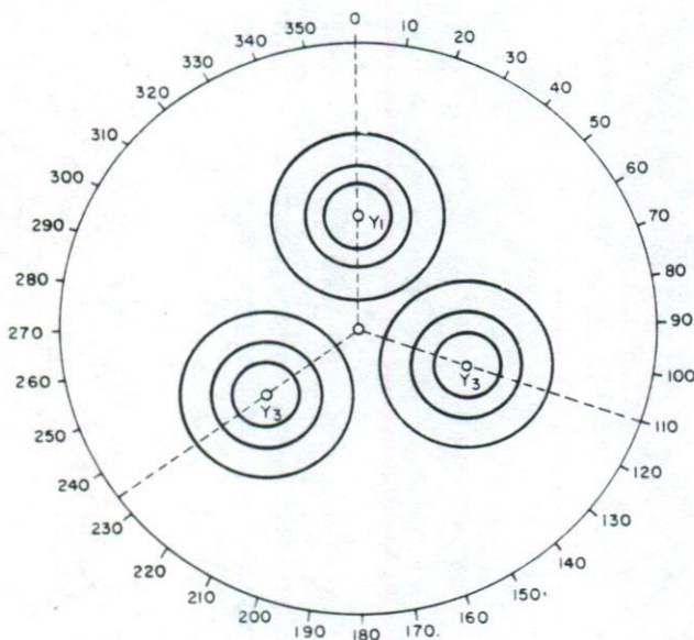
Fig. 39. PRD-PSD scan (vertical), 2-3/8 by 5 in. collimator scan of W68.
